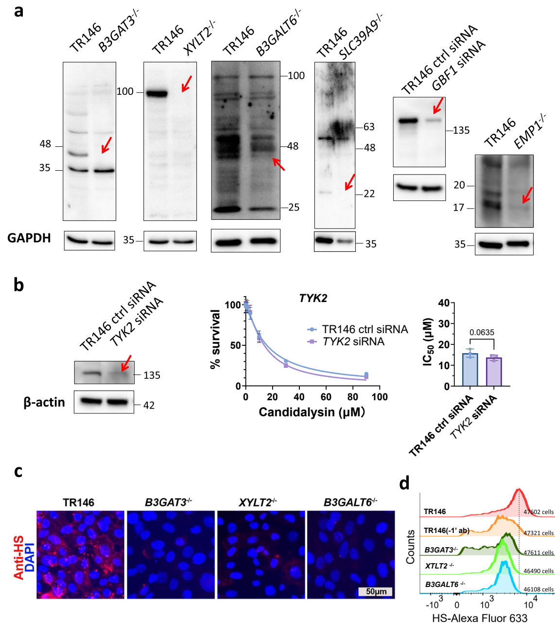
Extended Data Fig. 2 | Immunoblots and immunofluorescence images of gene knockouts and knockdowns. a , Immunoblots for B3gat3, Xylt2, B3galt6, Slc39a9 and Gbfl in the corresponding CRISPR knockout cells or siRNA knockdown cells. Arrows indicate the target proteins. Numbers indicate molecular mass. b , TYK2 siRNA knockdown does not affect survival of oral epithelial cells after 6-h of candidalysin exposure. The left panel shows a representative Tyk2 immunoblot. The middle panel shows the survival (measured by an XTT assay) of epithelial cells exposed to the indicated concentrations of candidalysin. The plots represent the combined results
