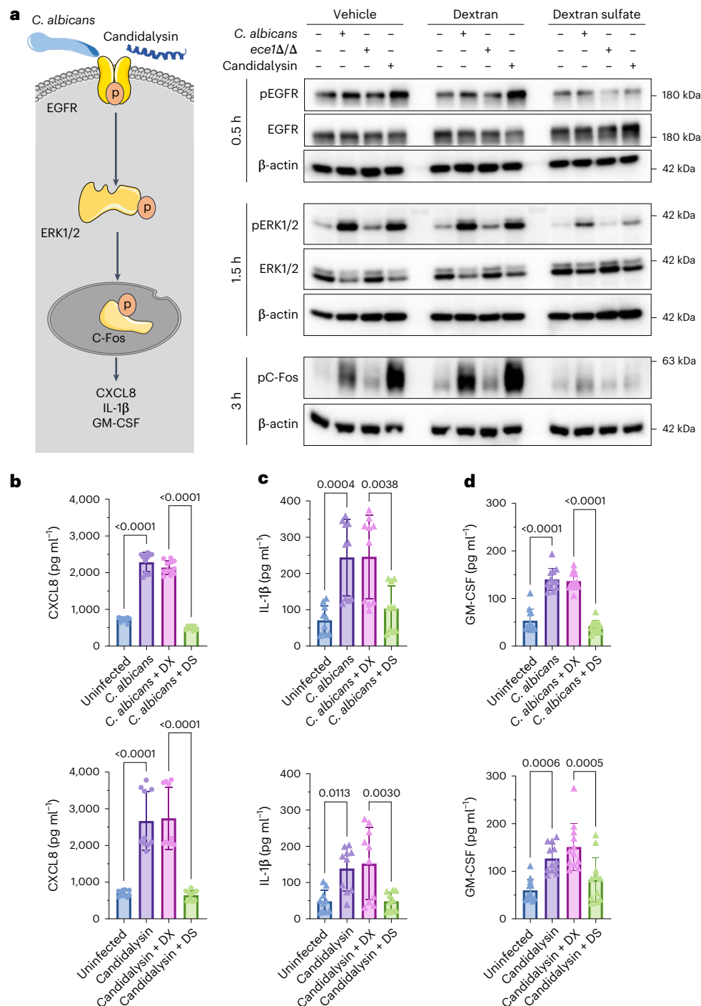
Fig. 5 | Sulfated GAGs mediate stimulation of oral epithelial cells by candidalysin and live C. albicans .
