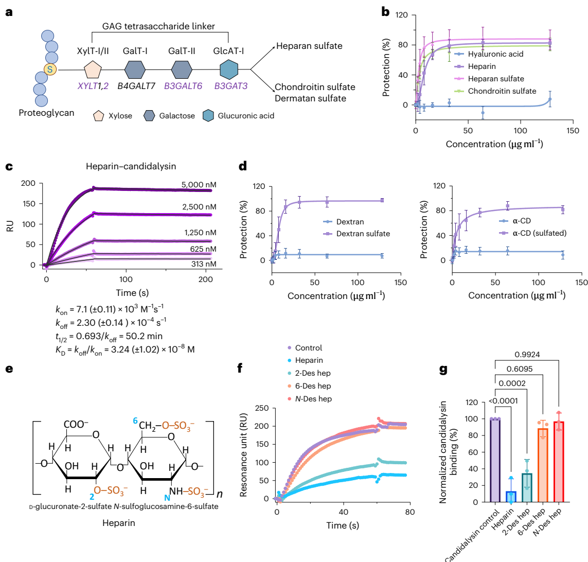
Fig. 2 | Sulfated GAGs and dextrin analogues bind to candidalysin and provide dose-dependent protection to epithelial cells against candidalysin-induced damage. a , Diagram illustrating the enzymes that catalyze the biosynthesis of the tetrasaccharide linker present in all GAGs. The genes that encode the enzymes are denoted under the monosaccharide, and the ones in purple are those identified by the CRISPR screen. b , Protection from damage caused by a 6 h exposure to 30 μM candidalysin provided by the indicated GAGs as measured by an XTT assay. The curves were generated from the data of three independent experiments, each performed in triplicate. Percentage protection was calculated as the normalized increase in host cell survival relative to control cells treated with candidalysin alone. c , SPR sensorgram of the interaction of candidalysin with heparin immobilized on the biosensor chip. The concentration of candidalysin used to generate each sensorgram is indicated on the graph. The binding kinetics ( k_{on} , association rate constant; k_{off} , dissociation rate constant; t_{1/2} , half-life; and K_D = k_{off}/k_{on} , binding equilibrium dissociation constant) were calculated from the global fitting of the five concentrations using a 1:1 Langmuir binding model. d , Protection from damage caused by a 6 h exposure to 30 μM candidalysin provided by dextran, dextran sulfate, α-cyclodextrin (α-CD) or sulfated α-cyclodextrin measured by an XTT assay. The curves were generated from the data of three independent experiments. e , Structure of heparin showing the location of the sulfate groups. f , Representative surface plasmon resonance sensorgrams showing the effects of 2-O-desulfated heparin (2-Des hep), 6-O-desulfated heparin (6-Des hep) and N-desulfated heparin (N-Des hep) on the interaction of candidalysin with heparin on the biosensor chip. g , Combined results of three independent experiments showing the inhibitory effects of the various desulfated heparins on the interaction of candidalysin with heparin. Results are mean ± s.d. P values were calculated using one-way ANOVA with Dunnett's multiple-comparison test.
